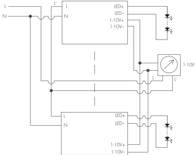
1-10V Connections
