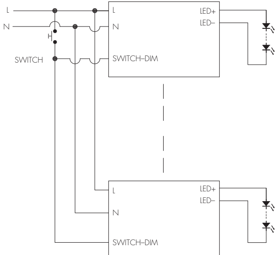
Switch-Dim Connections
