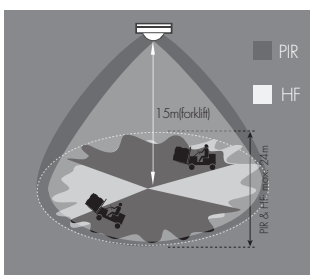
Detection pattern for forklift
