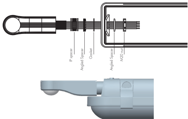
Typical Installation 2
