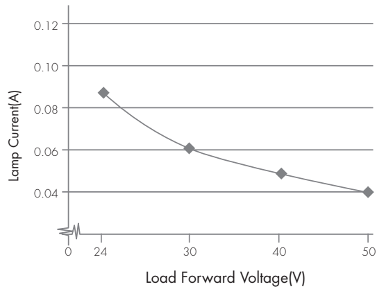
4W Output Current vs voltage
