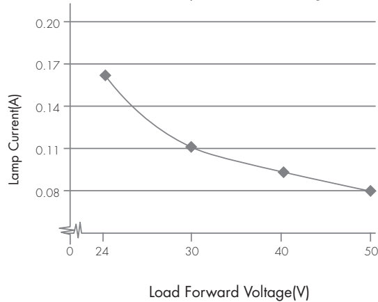
4W Output Current vs voltage
