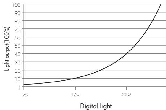
Dimming Characteristics
