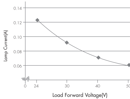
Dimming Characteristics
