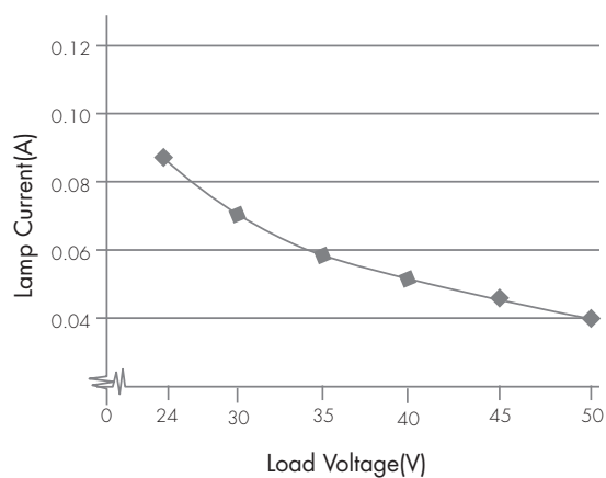
2W Output Current vs voltage
