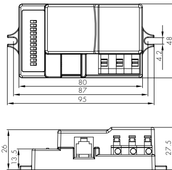
Mechanical structure (mm)
