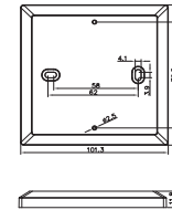
For the installation of a single switch
