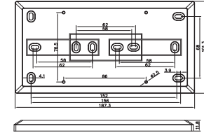
For the installation of double switches
