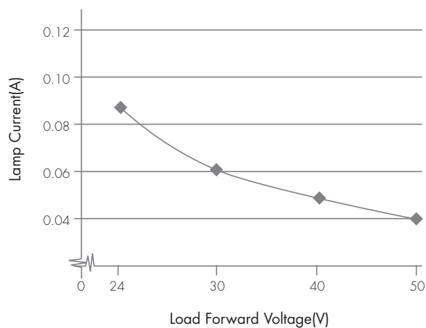
2W Output Current vs Forward Voltage
