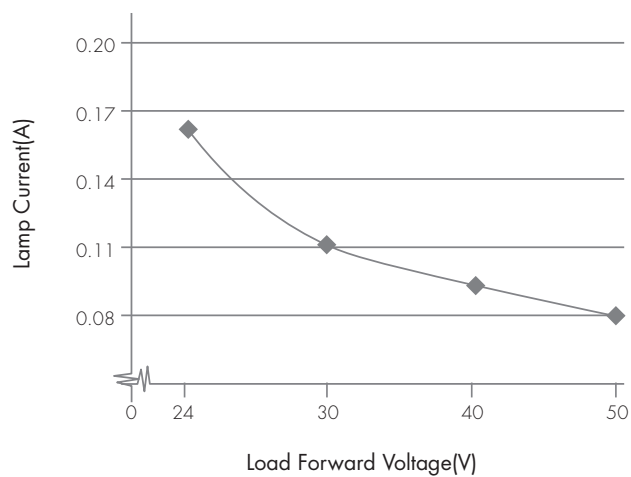
4W Output Current vs Forward Voltage
