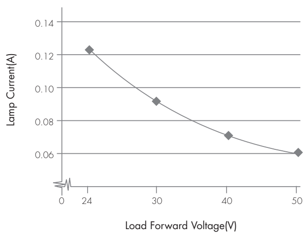
3W Output Current vs Forward Voltage
