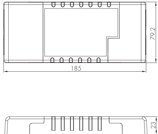
Stand-alone installation
