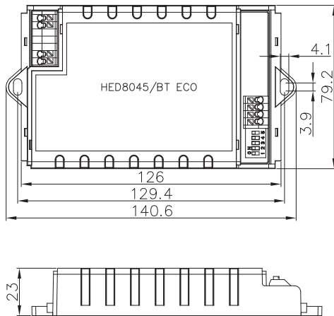
Built-in installation
