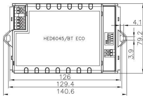
Built-in installation
